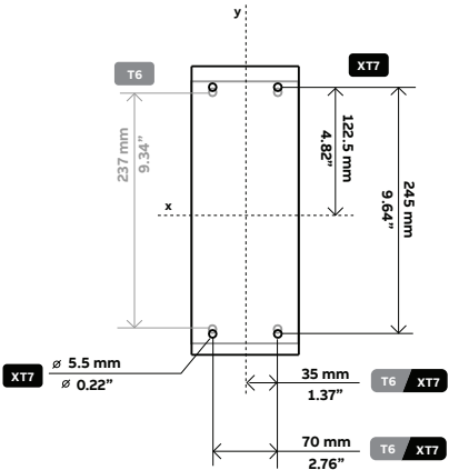
T6/XT7 FRAME SIZE FRONT COMPARISON
