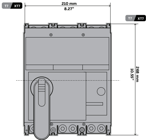
T7/XT7 FRAME SIZE FRONT COMPARISON
