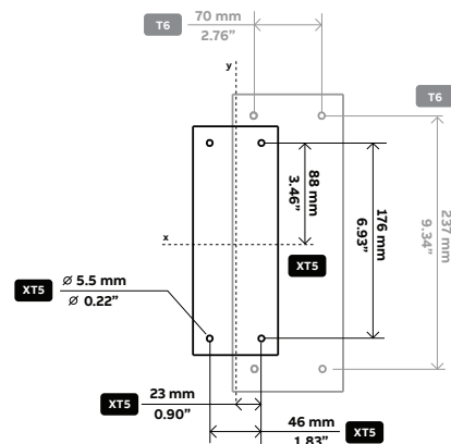
T6/XT5 FRAME SIZE FRONT COMPARISON
