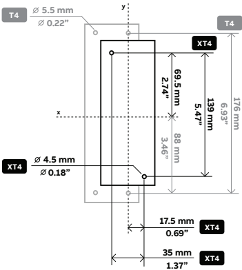
T4/XT4 FRAME SIZE FRONT COMPARISON
