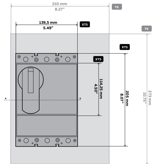
T6/XT5 FRAME SIZE FRONT COMPARISON
