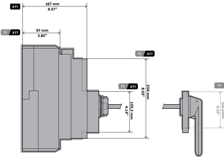
T7/XT7 FRAME SIZE DEPTH COMPARISON
