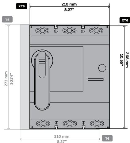
T6/XT6 FRAME SIZE FRONT COMPARISON
