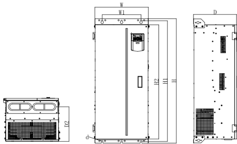
(e) Appearance of EM730-250-3 inverters
