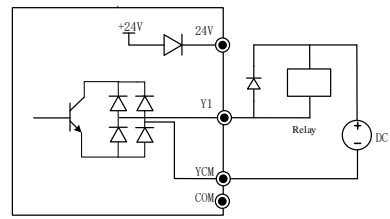
b: Use of external power supply NPN
