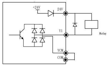
a: Use of internal power supply NPN
