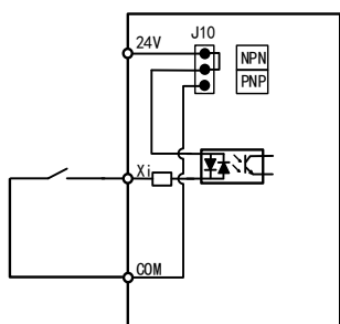
a: Use of internal power supply in NPN mode
