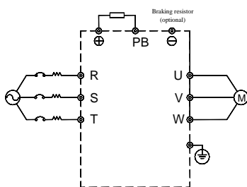
Fig.3-3 Standard Wiring of Main Circuit
