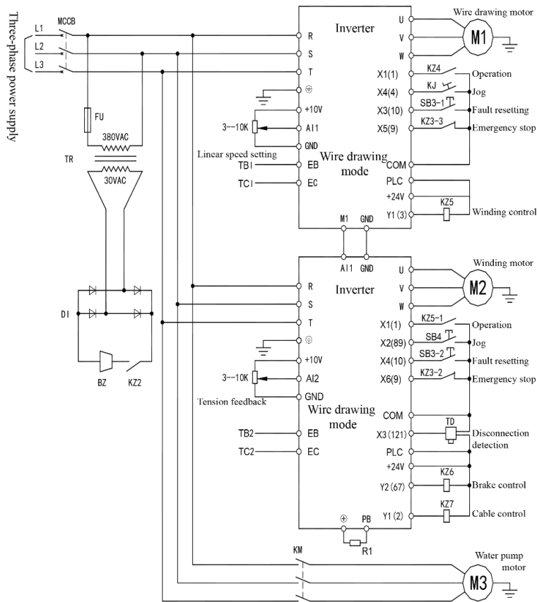
Wiring diagram of double-frequency wire drawing machine:
