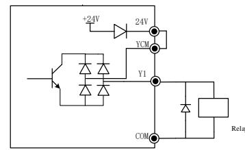
a: Use of internal power supply PNP
