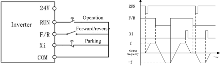
(c) Wiring diagram of three-line control (F00.03=3) (d) Forward/reverse running logic
