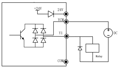
b: Use of external power supply PNP
