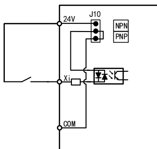
b: Use of internal power supply in PNP mode
