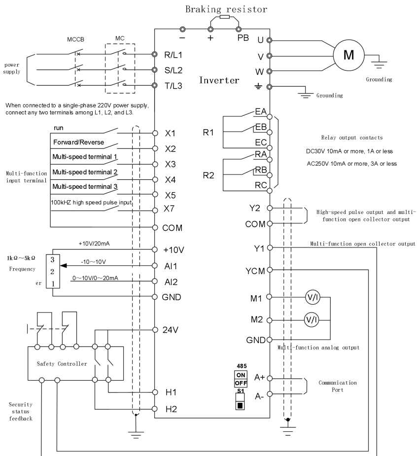
Figure 1 Control circuit wiring diagram
