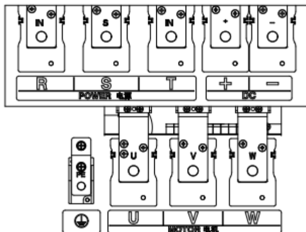
(g) EM730-185-3~EM730-250-3
