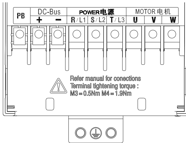
b) EM730-2R2-3B~EM730-4R0-3B
