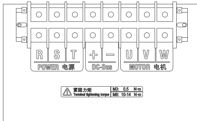
e) EM730-045-3~EM730-110-3
