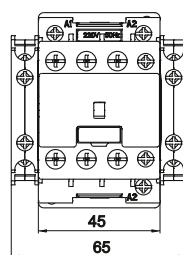
CNN 18+2xBP3
